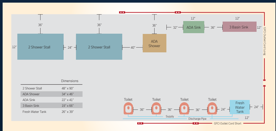
Example of Shower/Latrine Layout
